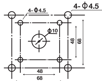
OVERSIZE PANEL MOUNTING DIMENSION DIAGRAM
