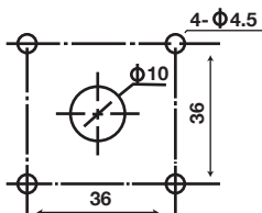
SMALL PANEL MOUNTING DIMENSION DIAGRAM
