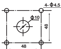
BIG PANEL MOUNTING DIMENSION DIAGRAM
